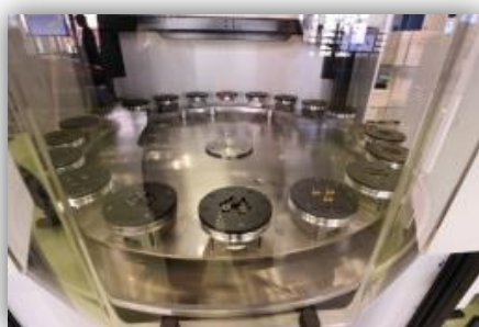
Magazine WorkPalCompact 12 positions Matrix
