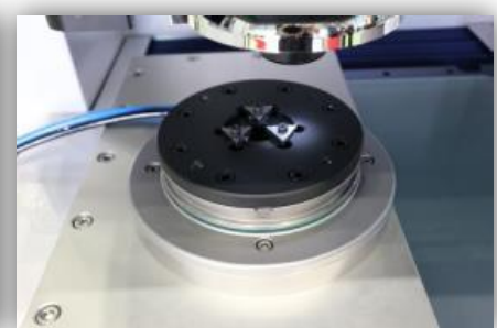
Matrix pallet special made for clamping 3 workpieces
